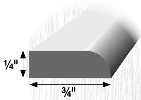
Scribe 48" Strips
